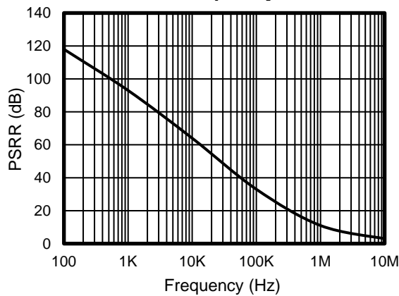
Figure 5. Power-Supply Rejection Ratio vs Frequency
