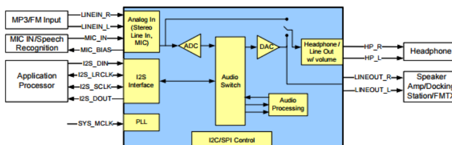
Figure 1. SGTL5000 Simplified Application Diagram
