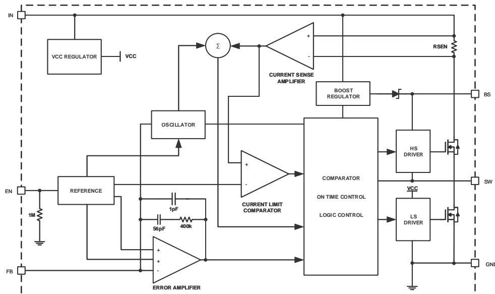
RY3835 Block Diagram
