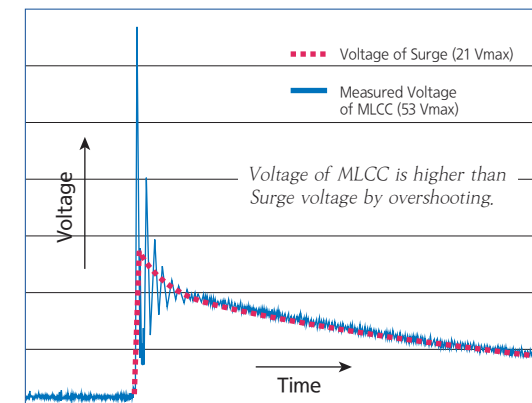
[ Example of Surge applied to MLCC ] * Simulation for ESD 8kV
