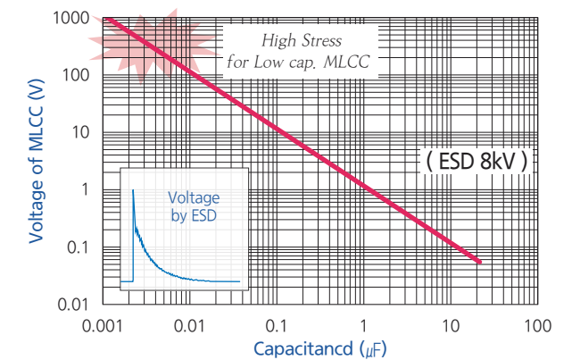
[ Example of ESD applied to MLCC ]
