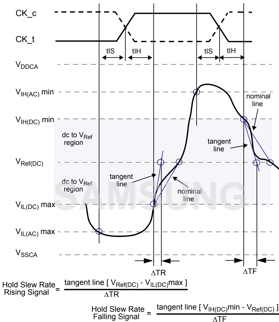
Figure 18. Illustration of tangent line for hold time t_{HH} for CA and CS_n with respect to clock
