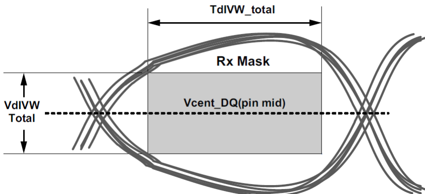
Figure 33. DQ Receiver (Rx) mask
