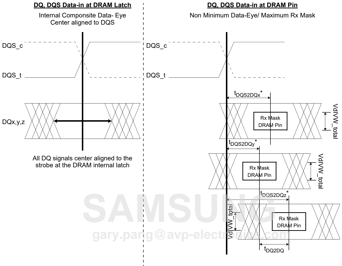
Figure 35. DQ to DQS t_{DQS2DQ} & t_{DQ2DQ} Timings at the DRAM pins referenced from the internal latch
