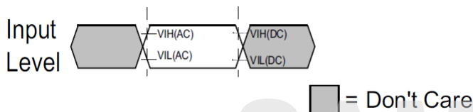
Figure 3. LPDDR4X Input AC timing definition for CKE 1-1). AC level is guaranteed transition point. 1-2). DC level is hysteresis.
