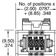
UMPC-03-X-XX-P-XX.X SHOWN
