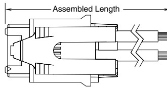
UMPC-04-X-XX-M-XX.X SHOWN
