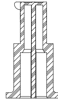
SECTION "C"-"C"
