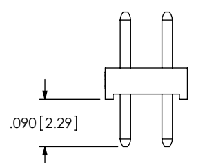
IN PROCESS 1 SCALE 4:1
