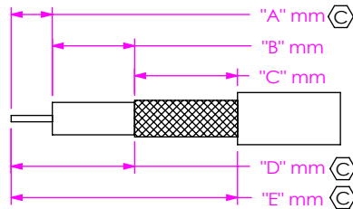
FIG 2 CABLE STRIPPING DIMENSIONS PER CONFIGURATIONS (SEE TABLE 1)(SEE NOTES 12,13,14,15)
