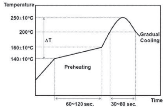
Infrared Reflow
