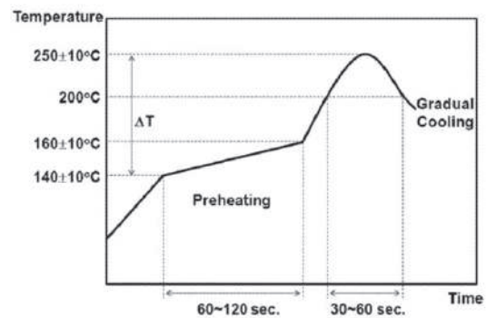
Infrared Reflow
