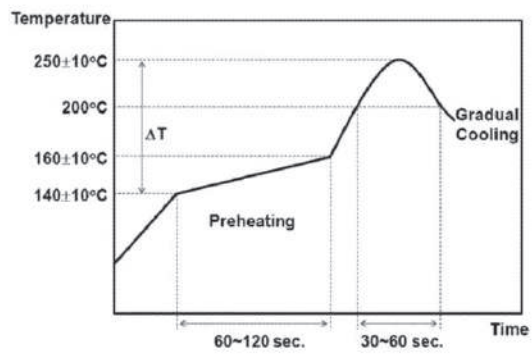
Infrared Reflow
