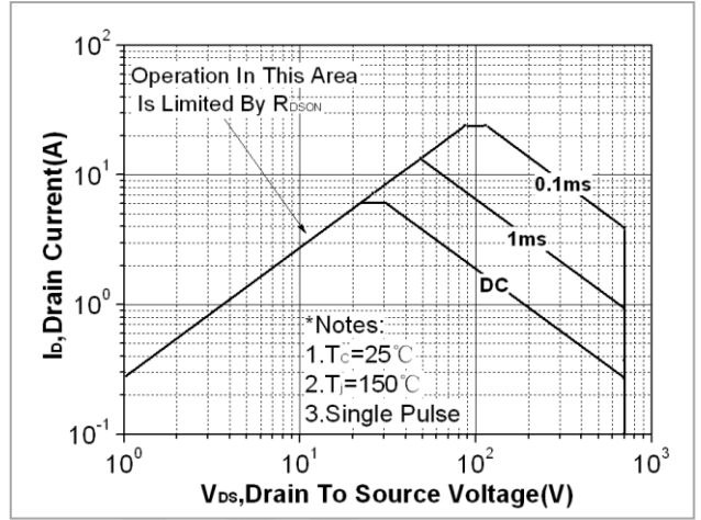
Fig. 14. Maximum safe operating area(TO-220)
