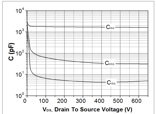
Fig.12. Capacitance Characteristics
