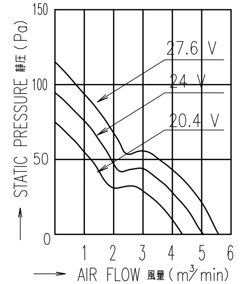
PERFORMANCE CURVES 風量-静圧特性例
