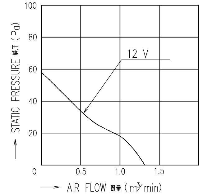
PERFORMANCE CURVES 風量-静圧特性例
