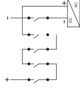
590.DCGE0820 - (5 POLES IN SERIES) - 4 JUMPERS SUPPLIED
