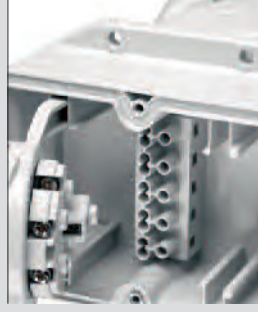
TOP version: entry-exit terminal board accessory.
