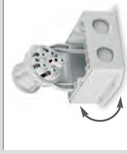
TOP version: reversible base and removable socket for easy wiring.
