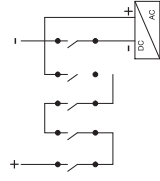
590.DCGE0820 - (5 POLES IN SERIES) - 4 JUMPERS SUPPLIED
