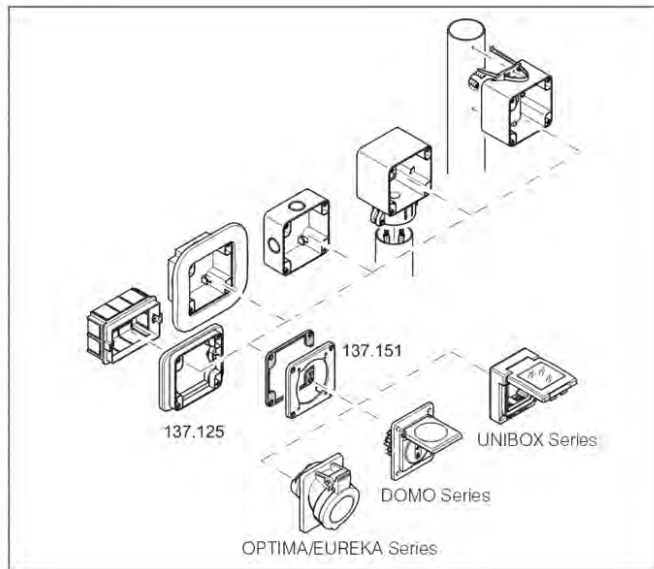
PROTECTA Series Cover for M95 boxes with 70x87mm predrilling
