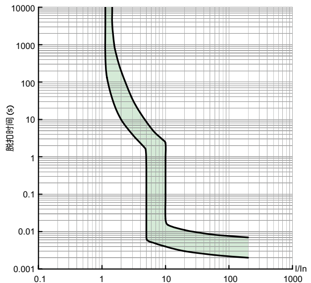
iDPNa/N/H, iDPNa-K C曲线
