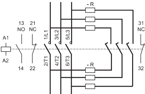
LC1D•K
