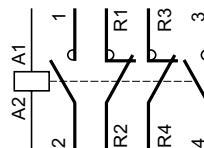
LC1E06...38008
