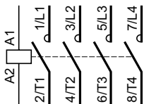
LC1E06...95004
