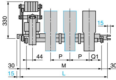
Single, 2 or 3-pole contactors LC1 B●31, B●32 or B●33
