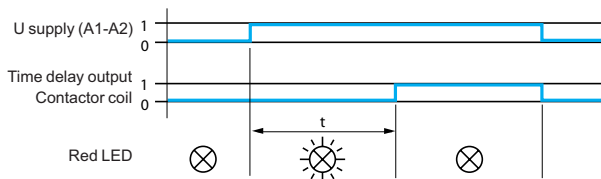
Electronic on-delay timer LA4 DT
