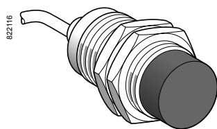
XS230BL●●L●
