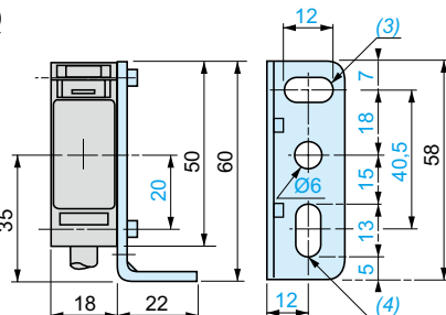
Bracket fixing (1)
