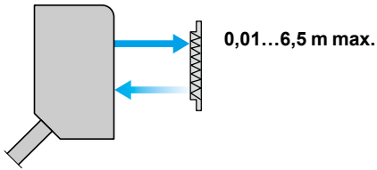
With reflector
