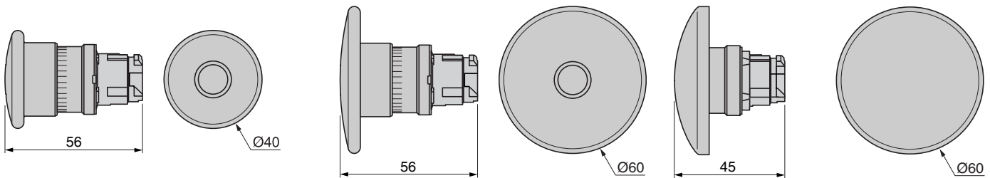
Turn to release ZB4-BS4●, BS834
