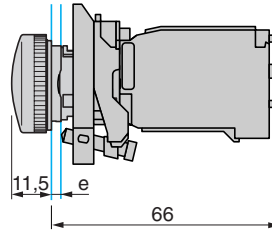
Via integral transformer ZB4-BV3, 4 + ZB4-BV0●●
