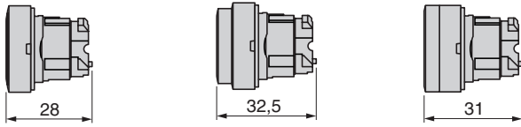
Heads for pushbuttons, spring return ZB4-BA●, BA●●●, ZB4-BA●8 ZB4-BL●, BL●●●
