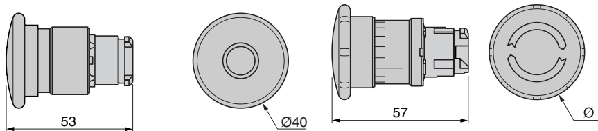
Turn to release ZB4-BS4●, BS834
