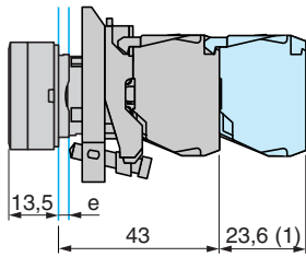
Illuminated pushbuttons Integral LED ZB4-BW0●●● + ZB4-BW3●●● + ZBE-●●●
