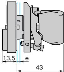
Double-headed pushbuttons with pilot light Integral LED ZB4-BW0●●● + ZB4-BW8●●●●●
