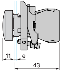
Pilot lights Integral LED ZB4-BVB●/BVG●/BVM● + ZB4-BV0●●
