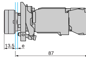
Illuminated selector switches Integral LED ZB4-BK1●●● + ZB4-BW0●●●
