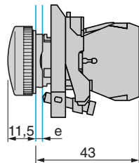
Direct supply ZB4-BV6 + ZB4-BV0●●
