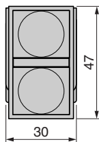
Double-headed pushbuttons with pilot light Integral LED ZB4-BW0●●● + ZB4-BW8●●●●●
