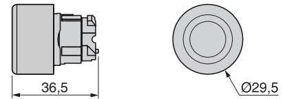
ZB4-BP●● ZB4-BP●S
