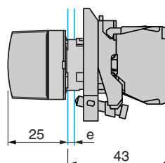
Illuminated selector switches Integral LED ZB4-BK1●●● + ZB4-BW0●●●
