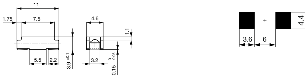
Soldering pads
