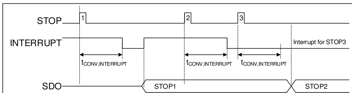
Figure 49: Conversion Latency
