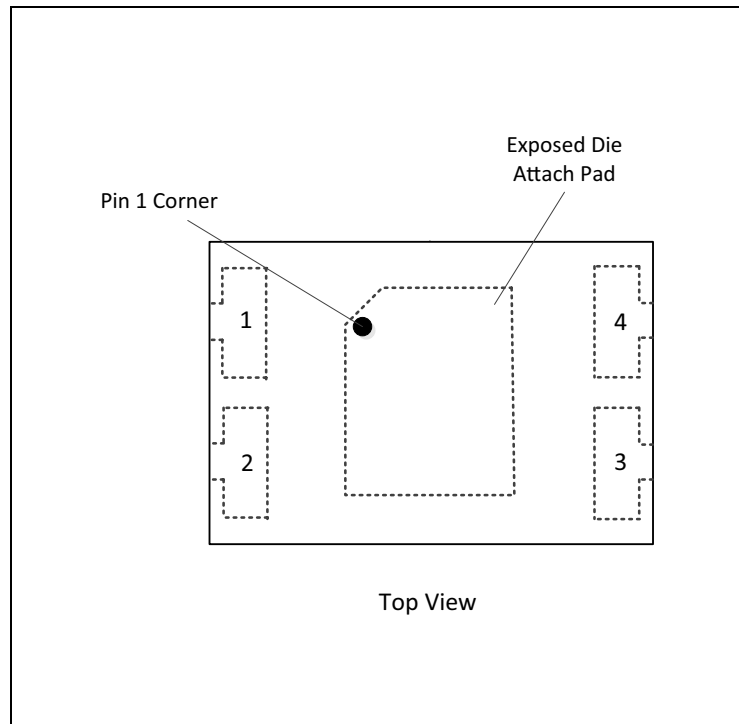
Figure 3: Pin Diagram
