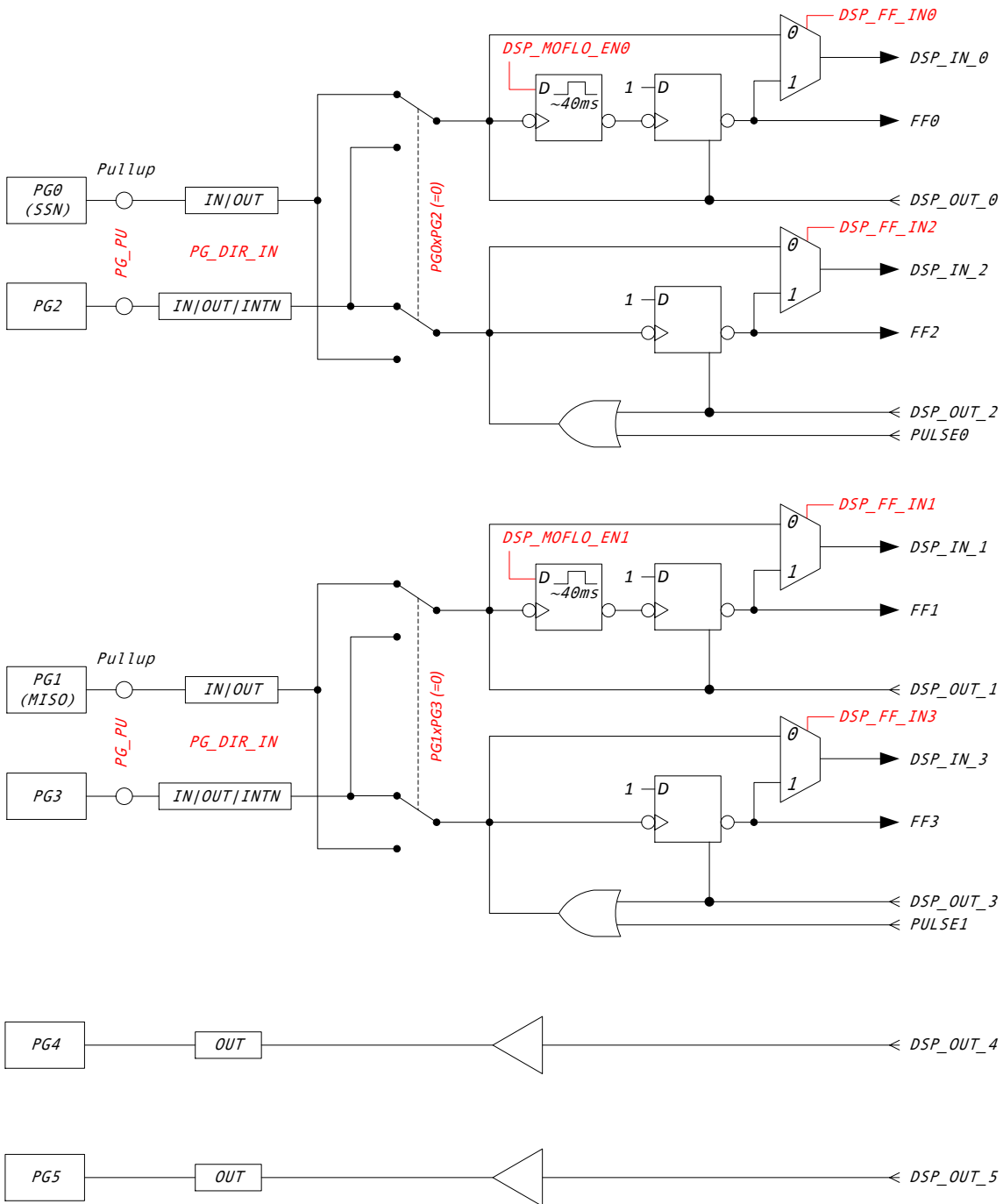
Figure 2-2 GPIO Assignment
