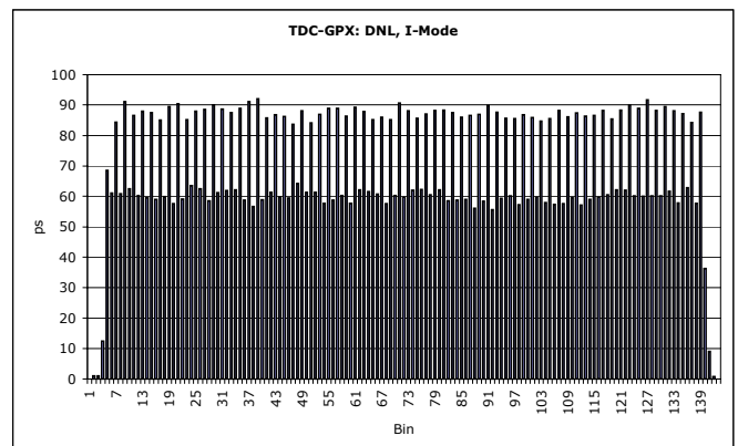
Figure 22: DNL
