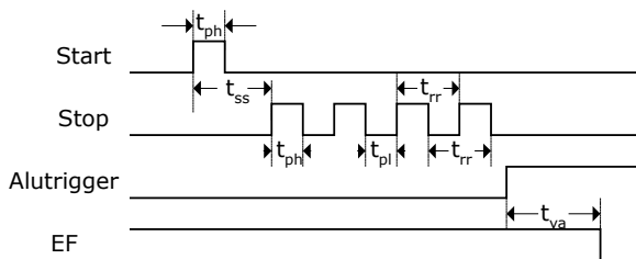
Figure 25. Measurement timings
