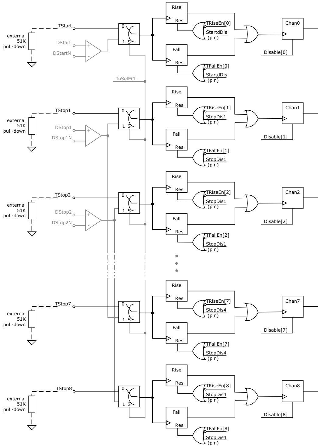
Figure 17: Input circuitry
