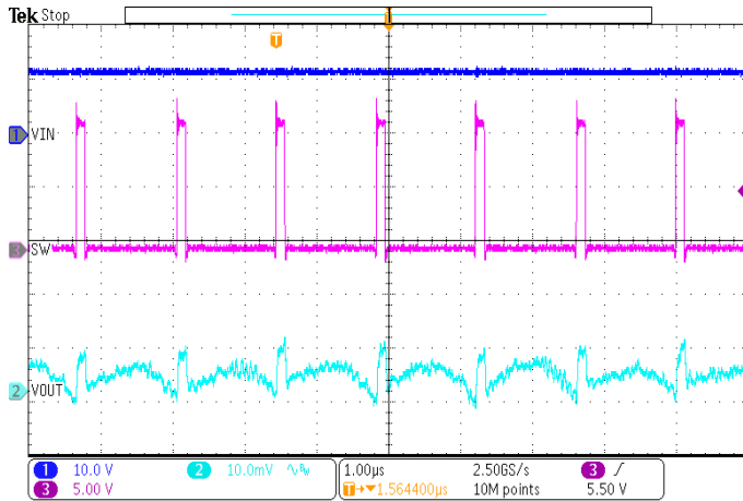
Figure 8. Switching Waveforms and Output Ripple ( IOUT=2A )
