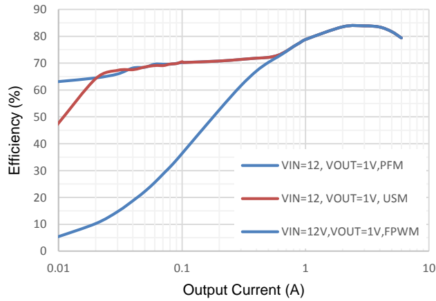
Figure 2. Efficiency vs Load Current, fsw=800kHz
