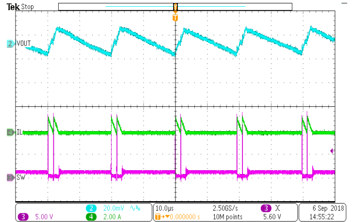
Figure 9. Switching Waveforms and Output Ripple in PFM ( IOUT=100mA )
