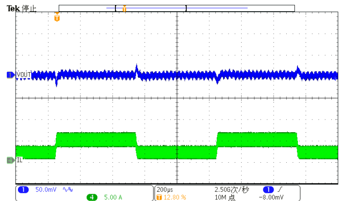
Figure 16. Load Transient (Vout=1V, Iout=1.5A to 4.5A)
