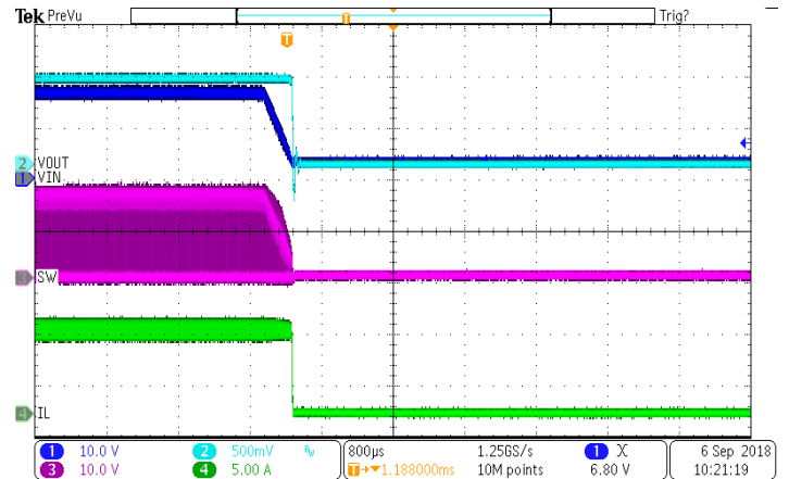
Figure 11. Power down
