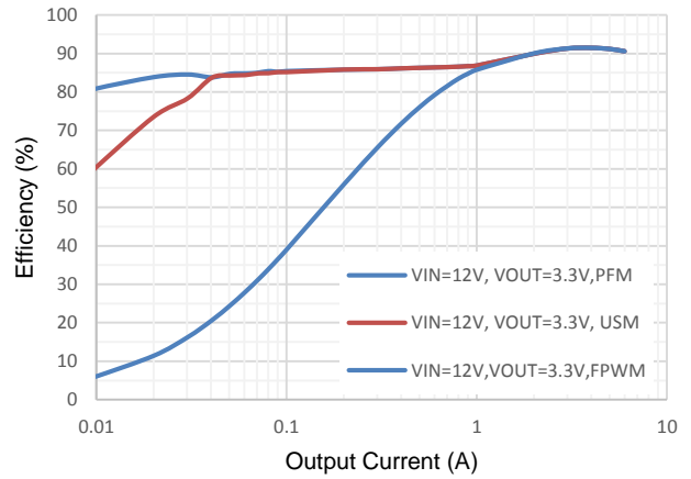
Figure 3. Efficiency vs Load Current, fsw=800kHz
