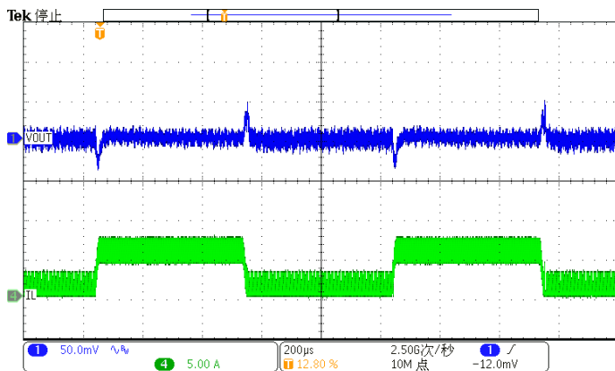
Figure 15. Load Transient (Vout=1V, Iout=0.6A to 5.4A)
