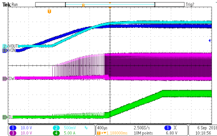
Figure 10. Power up
