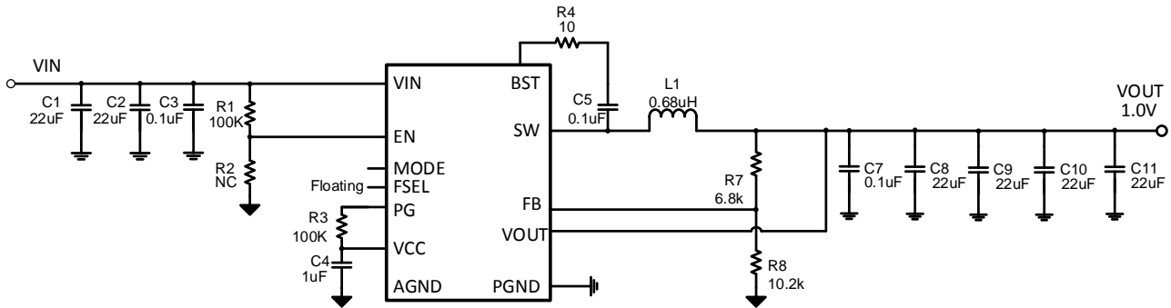
Figure 10. SCT2260A Design Example, 1V Output
