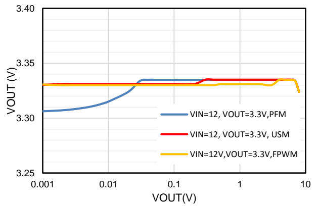
Figure 5. Load Regulation, fsw=800kHz
