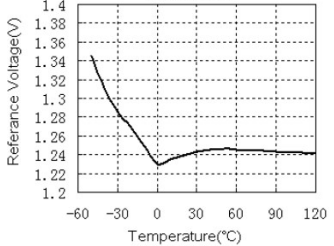
Reference Voltage VS Temperature (Iload=10mA)
