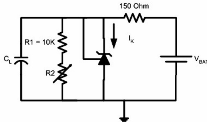
Test Circuit for V_{KA} = 2\text{V}, 3\text{V}
