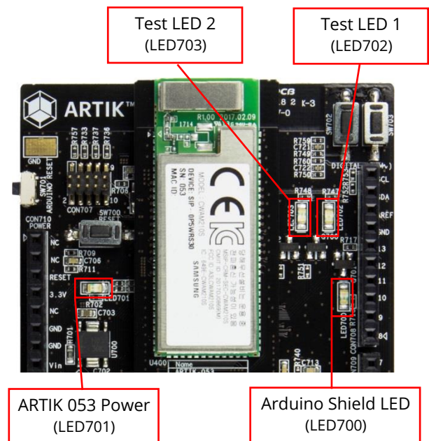
Figure 8. LED locations
