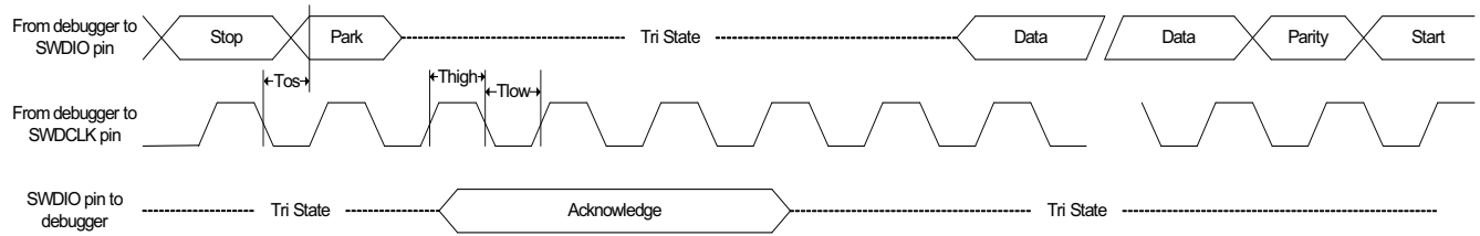
Figure 36-23. SWD Interface Signals
