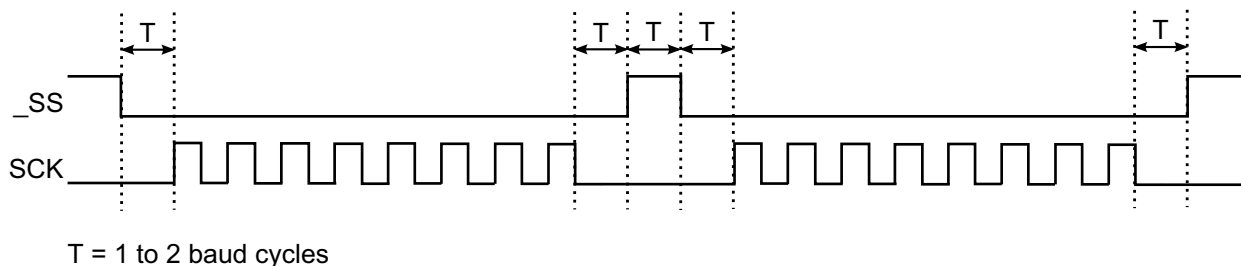
Figure 26-7. Hardware Controlled \text{\_SS}
