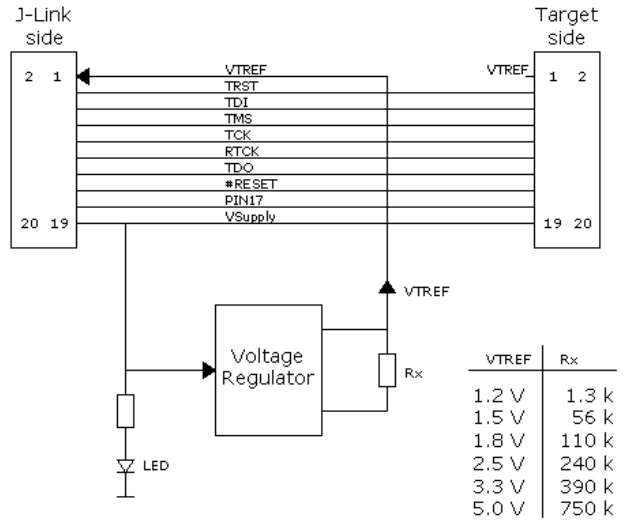
Block diagram of the J-Link Supply Adapter
