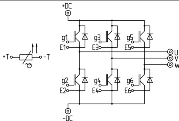
pinout, dimensions
