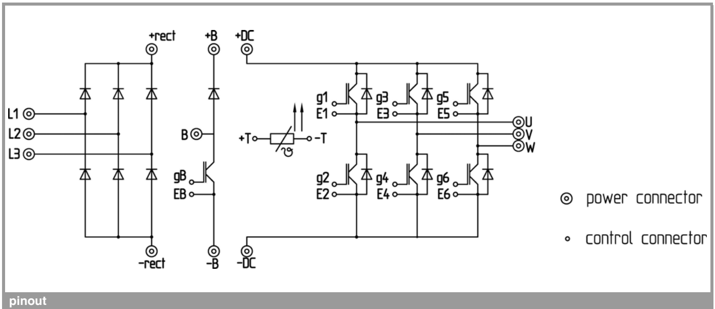
pinout, dimensions
