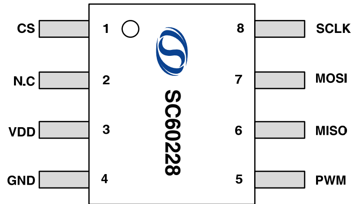
8-Pin SOP8 DC Package (Top View)
