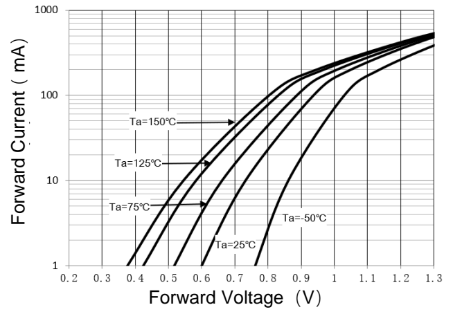
Fig 2. V_F characteristics
