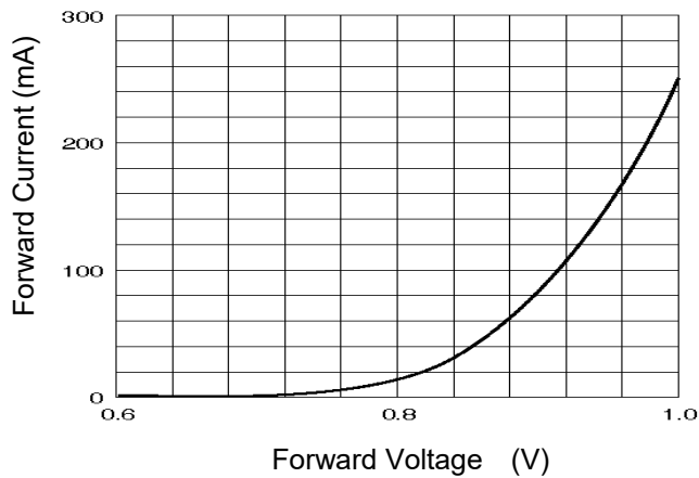
Fig 3. Forward Characteristics Curve
