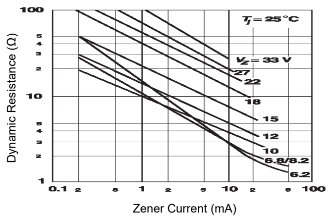
Fig 2. Dynamic Resistance vs.Zener Current
