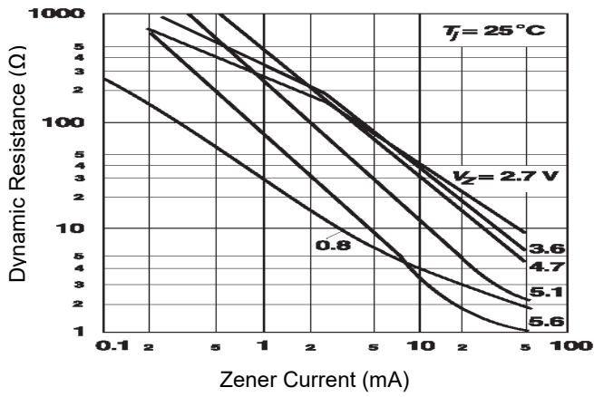
Fig 1. Dynamic Resistance vs.Zener Current
