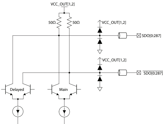
Figure 3-2: Trace Driver Output Equivalent Circuit (includes the MON0 & MON1 outputs)
