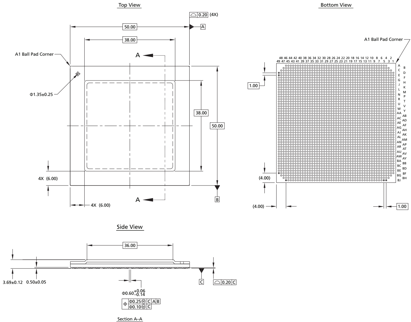
Figure 6-1: Package Dimensions
