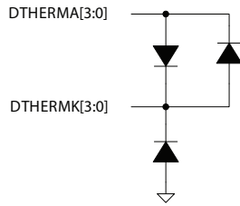
Figure 4-3: Temperature Sensors
