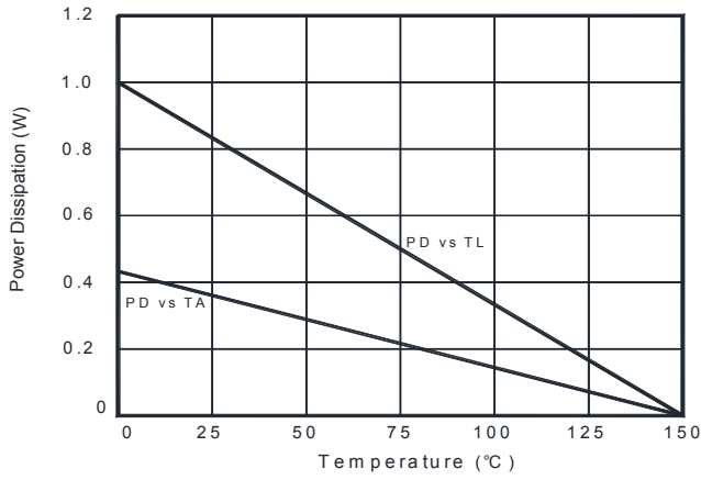
Fig 1. Power Dissipation vs. Temperature
