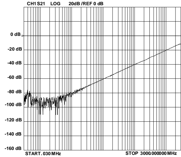
Analog Crosstalk
