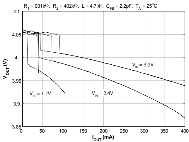
Load Regulation ( V_{OUT} = 4.0V )
