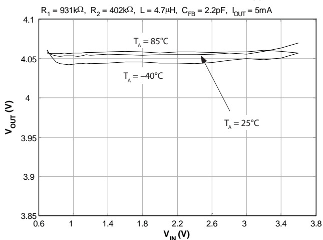
Line Regulation — PSAVE Mode ( V_{OUT} = 4.0V )
