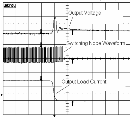
Load Transient Test ( V_{IN}=5V , V_{OUT}=1.2V , I_{OUT}=3A to 0A , L_{OUT}=1.0\mu H , C_{OUT}=2x22\mu F , Channel 1: 50mV/Div, Channel 2: 5V/Div, Channel 4: 2A/Div, Time: 20µs/Div)
