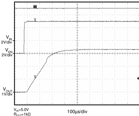
Start Up (Enable)( V_{OUT}=3.3\text{V} )
