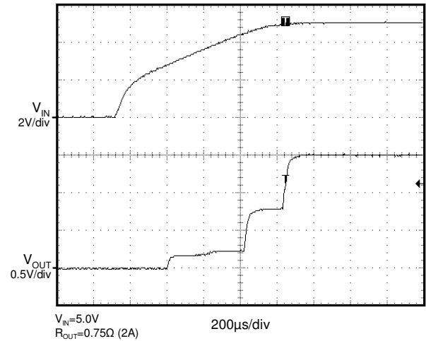
Start Up (Power up V_{IN} )( V_{OUT}=1.5\text{V} )
