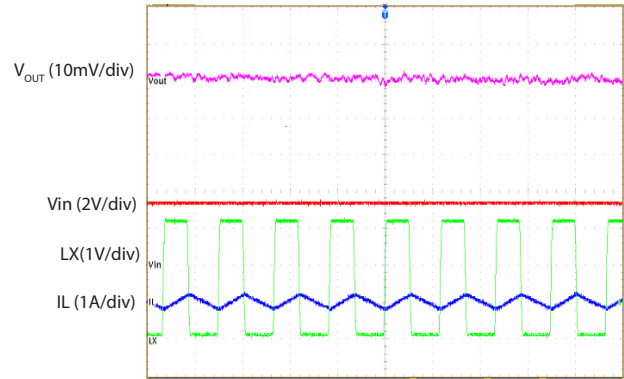
Vout Ripple ( V_{in}=3.3\text{V} , V_{OUT}=1.5\text{V} )@ 0A Load
