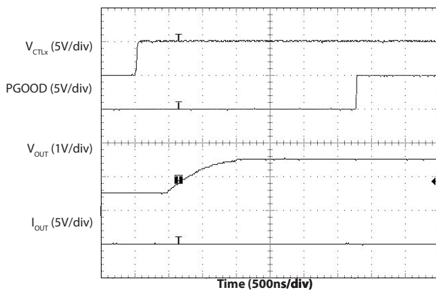
Start Up into Pre-Biased Output ( V_{OUT} = 1.5\text{V} )
