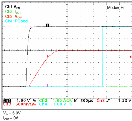
Start Up ( \text{CTL}_X ) — No Load
