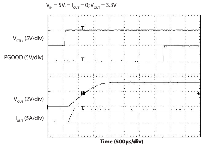
Start Up ( \text{CTL}_X ) — Full Load
