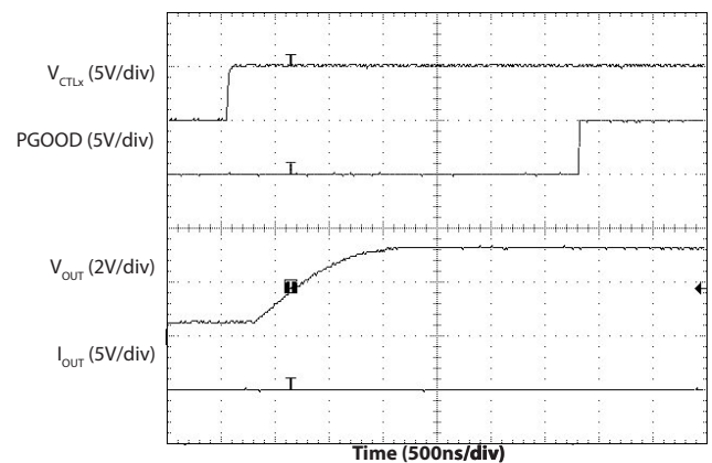
Start Up into Pre-Biased Output ( V_{OUT} = 3.3\text{V} )
